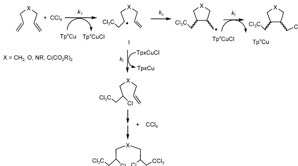
Scheme 7. Kharasch addition of \text{CCl}_4 to 1, \omega -dienes catalyzed by \text{Tp}^X\text{Cu}(\text{I}) complexes.
