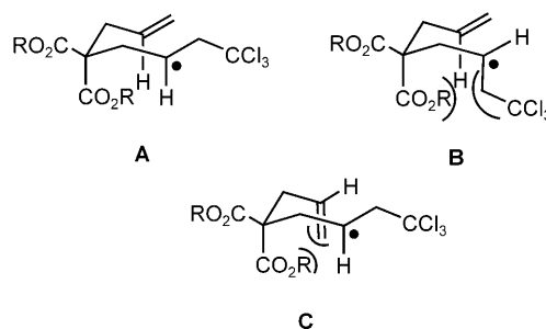
Scheme 6. Transition states for the cyclization reaction.
