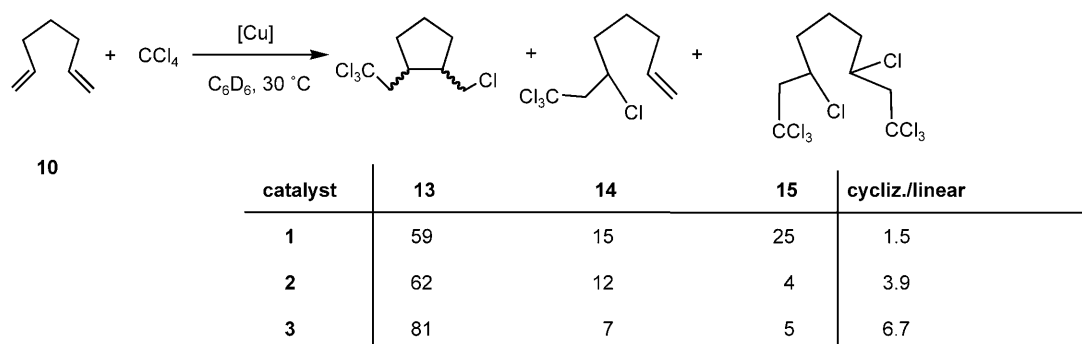
Scheme 4. Ring-closing Kharasch addition of \text{CCl}_4 to 1, \omega -dienes catalyzed by \text{Tp}^x\text{Cu(I)} complexes.
