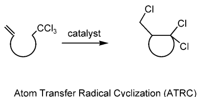
Scheme 1. ATRA and ATRC reactions.
