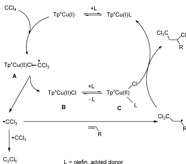
Scheme 5. Mechanistic proposal for ATRA reactions catalyzed by \text{Tp}^x\text{Cu} complexes.
